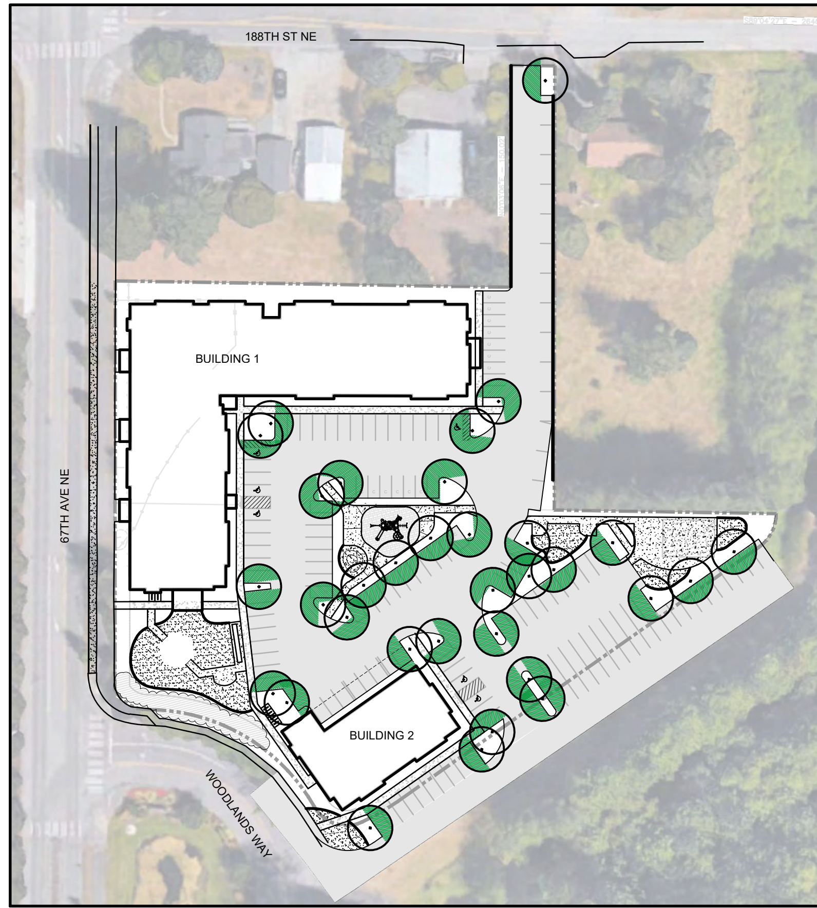
VEHICLE ACCOMMODATION SHADE AREA NO SCALE
